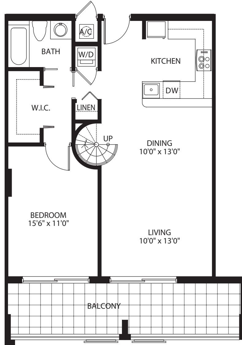
Lower Level
