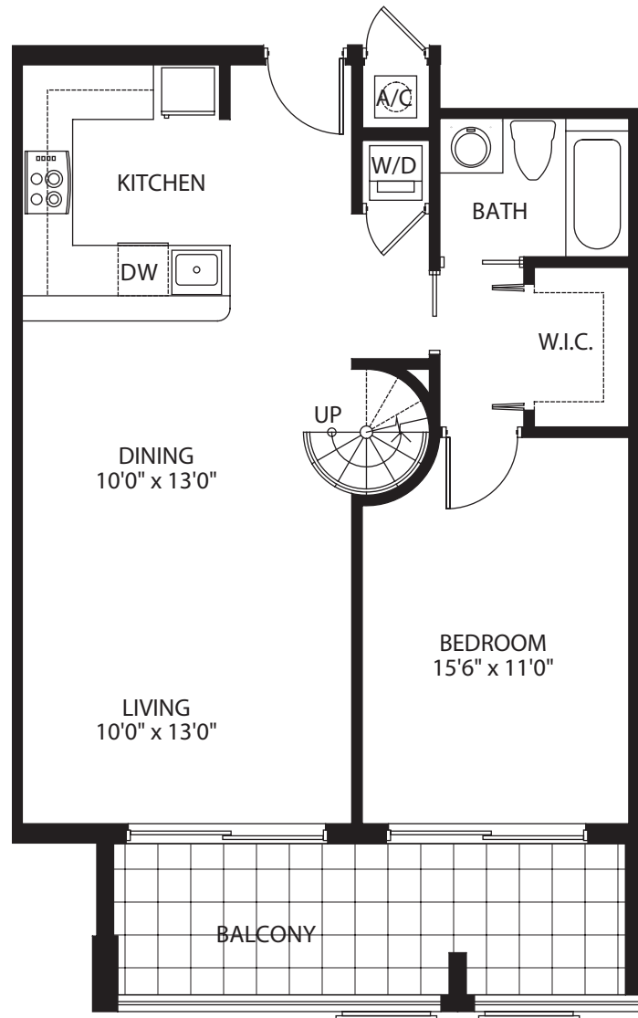
Lower Level
