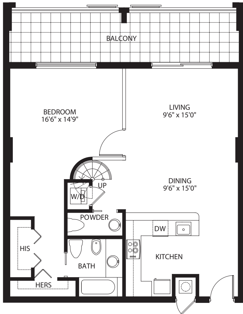
Lower Level
