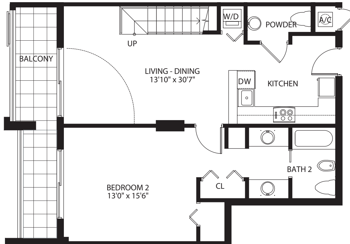
Lower Level
